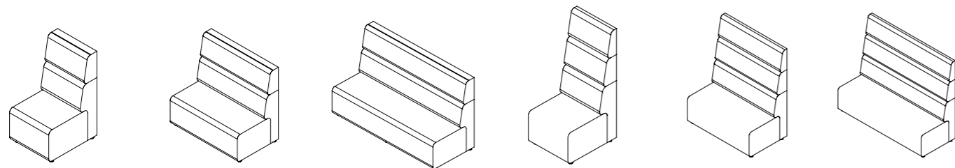
ALL07 ALL08 ALL09 ALL10 ALL11 ALL12 W 600 D 735 H 1150 W 1200 D 735 H 1150 W 1800 D 735 H 1150 W 600 D 735 H 1500 W 1200 D 735 H 1500 W 1800 D 735 H 1500
