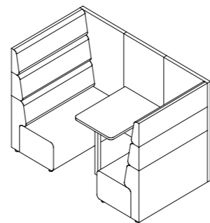
ALL15 W 2230 D 1250 H 1500
